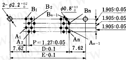
Mating Side
